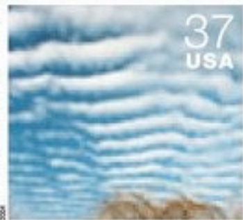
Altopcumulus undulatus
