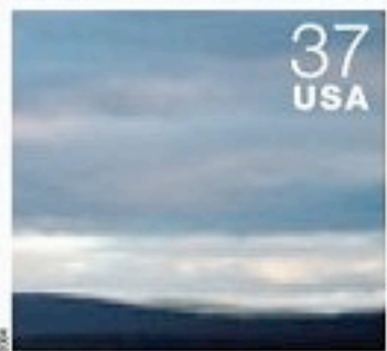
Stratocumulus undulatus
