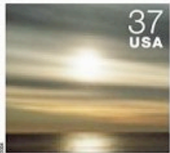
Altostratus translucidus
